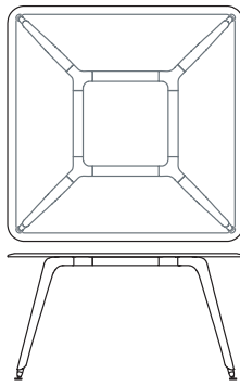
Square meeting table 1BE0401: L 55 D 55 H 29½ 1BE0403: L 63 D 55 H 29½ 1BE0405: L 63 D 55 H 29½
