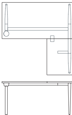
Free-standing single desk with 80x60 right return 1BE1021: L 63 D 64 H 29½ 1BE1023: L 71 D 64 H 29½
